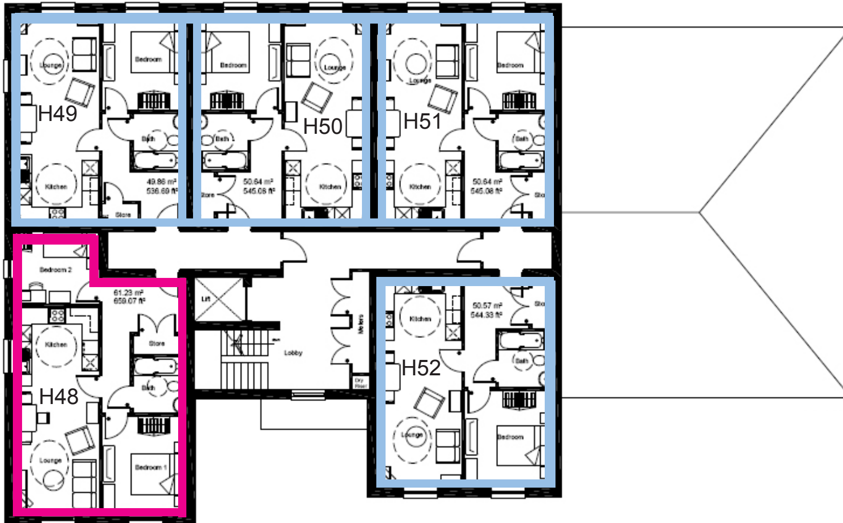
Third Floor - Plots H48 to H52
